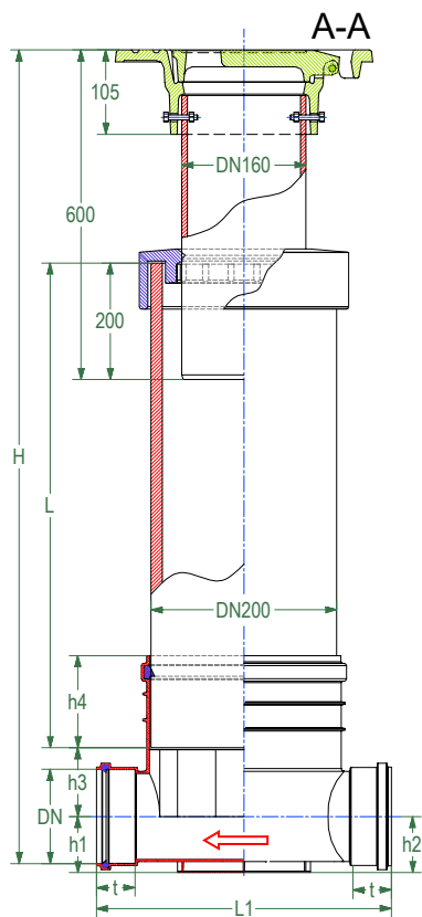
DN200 BASE, TYPE 1B
