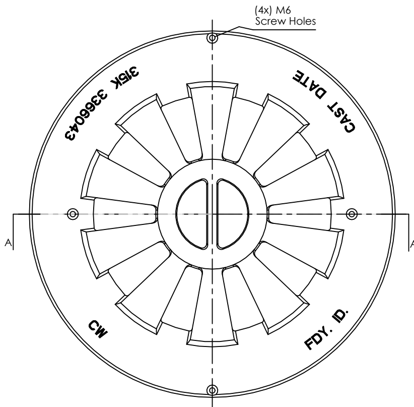
PLAN VIEW
