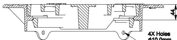
SECTION T-T
