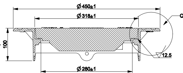
SECTION X-X
