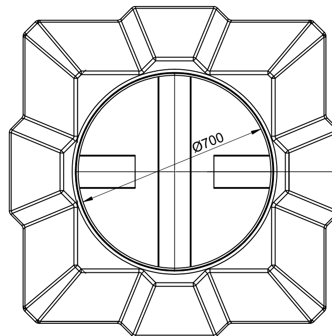
DETAIL D
